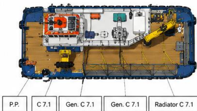
Top Deck
