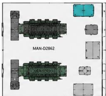
Engine Room
